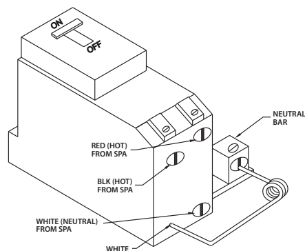
TYPICAL GFCI ISOMETRIC VIEW
